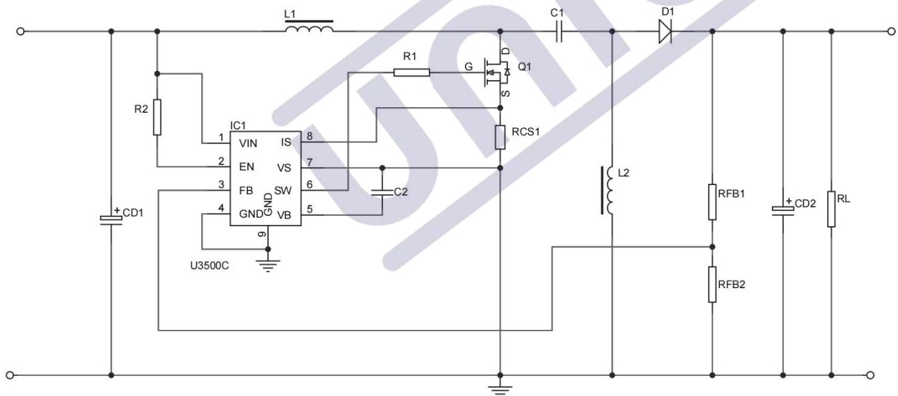
Application of step-up and step-down voltage.
